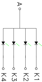
LED CIRCUIT
