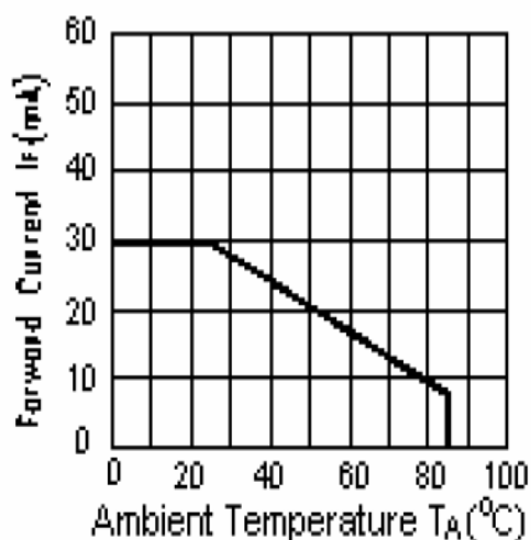
I f LED VS TEMP
